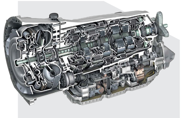
725.0 Series Cutaway
